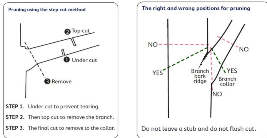
Figure 6.1-3: Correct pruning techniques
