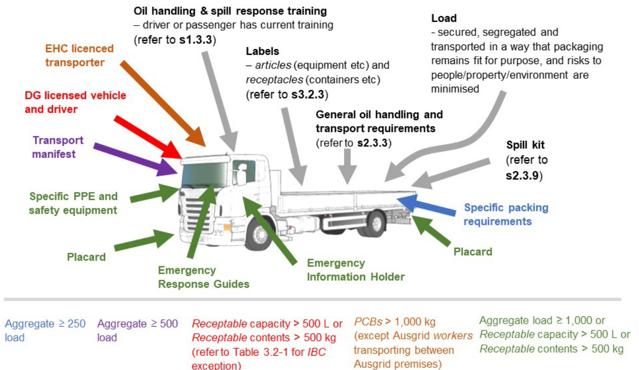
Figure 3.2-2: Summary of requirements for transporting scheduled PCB
