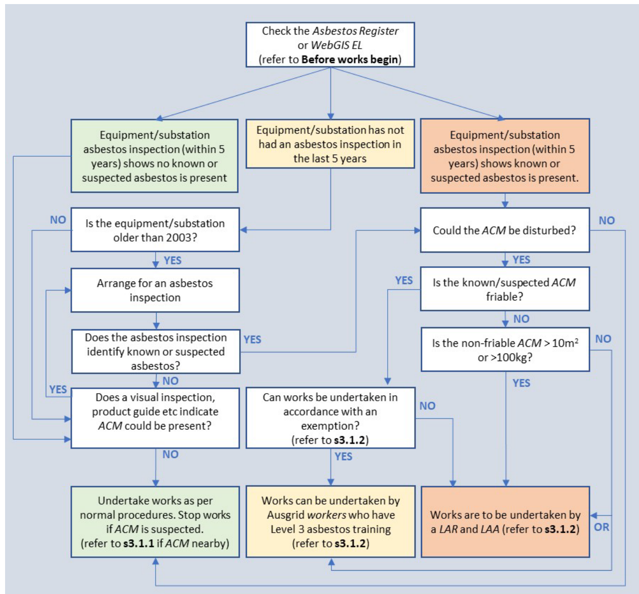
Figure 3.1-1: Process for working with asbestos
