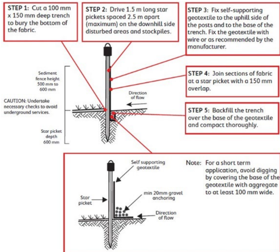
Figure 2.1-3: Sediment fence installation instructions
